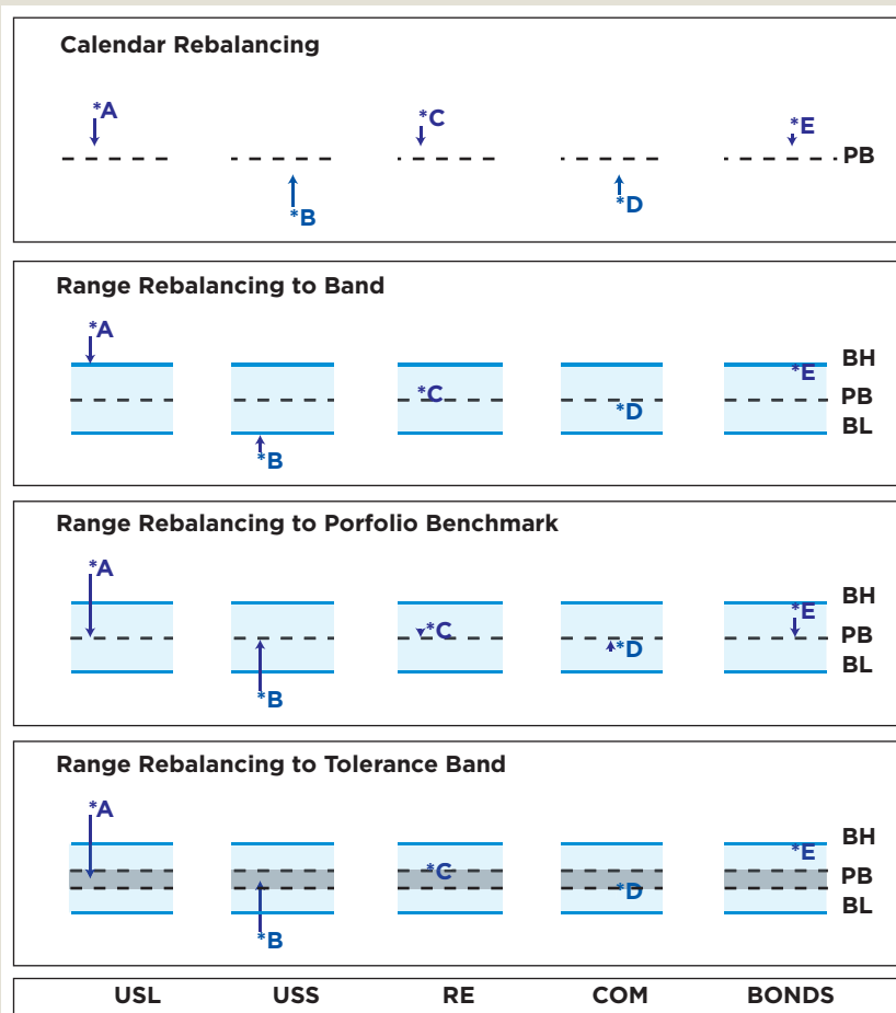
Figure 2: Rebalance Approaches
